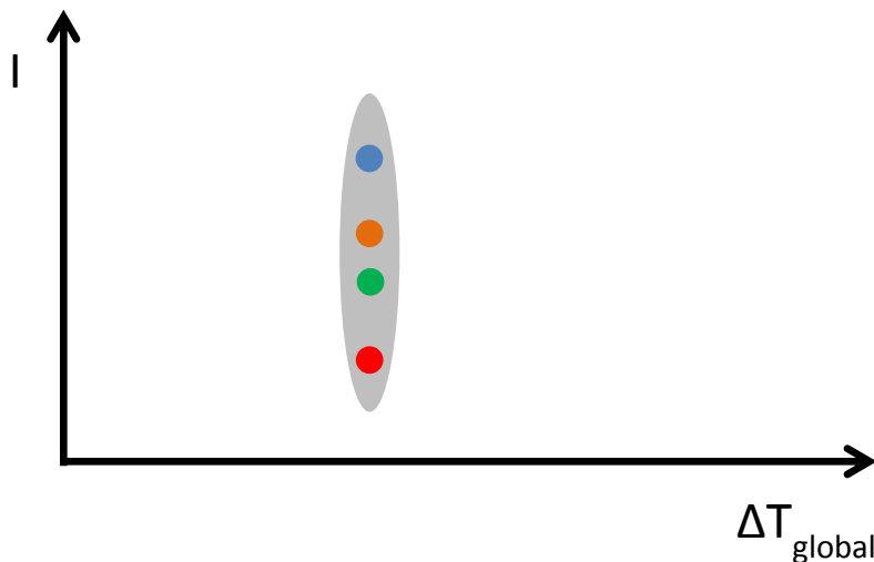
Figure 2 Schematic plot of the climate impacts as projected for 1 impact model, 1 RCP and 4 different GCMs. The points do not correspond to a fixed time, only a fixed \Delta T_{\text{GMT}} . Only the start and end points of the line are for a common time.
