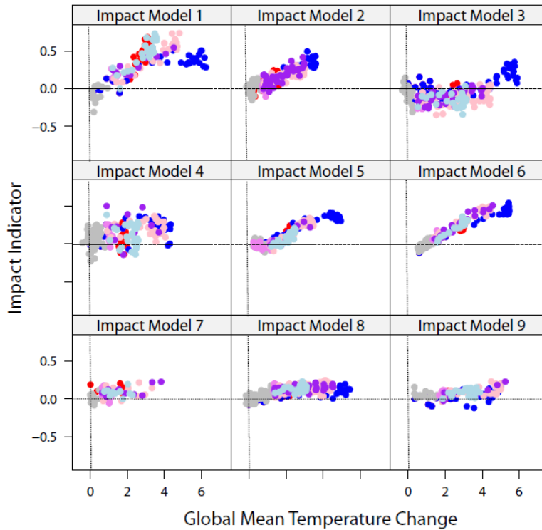
Figure 1. Example plot of changes in impacts as a function of global mean temperature change, assuming a minimal model set-up (one GCM, all RCPs, nine impact models). Each point represents a pair of annual values of global mean temperature change and associated impact indicator. Sub-panels show results for different impact models, and the color indicates different climate scenarios.
