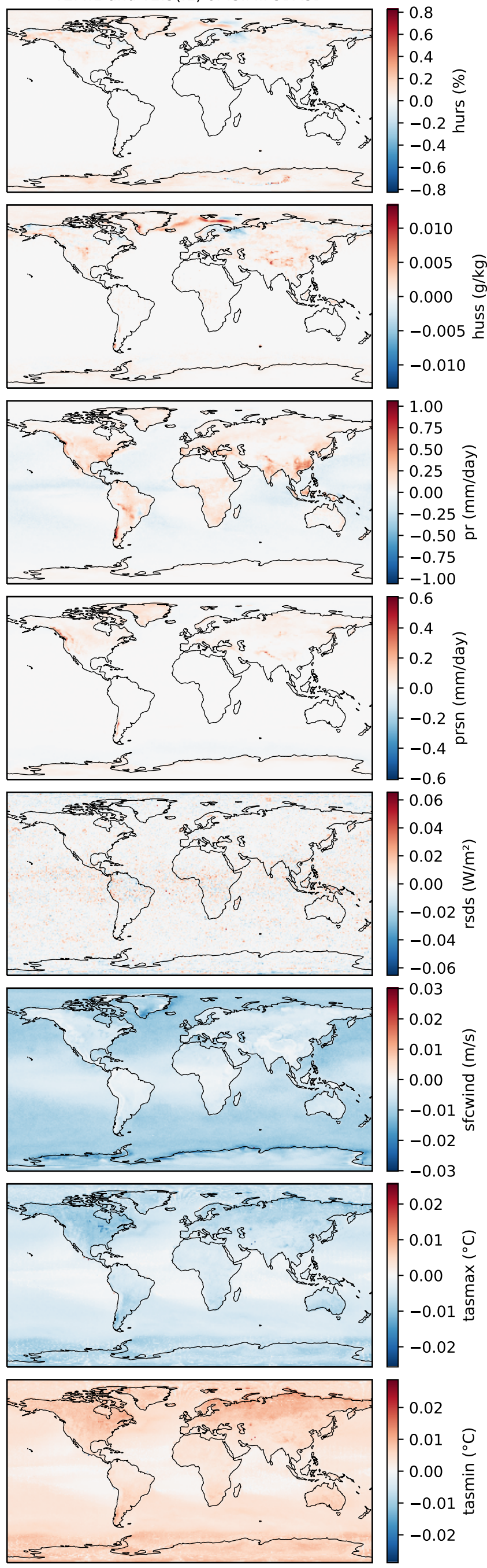
mean difference over 1850-2014 between data bias-adjusted with v2.4.1 and v2.3(.1) of ISIMIP3BASD
