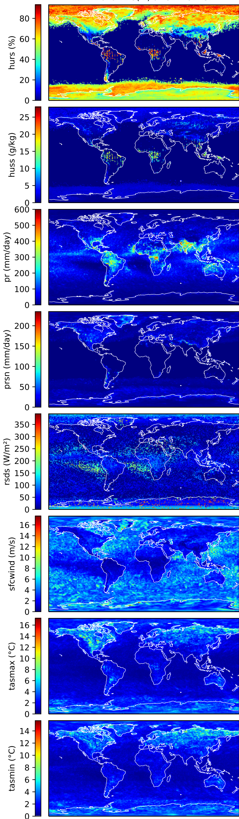
maximum absolute difference over 1850-2014 between data bias-adjusted with v2.4.1 and v2.3(.1) of ISIMIP3BASD
