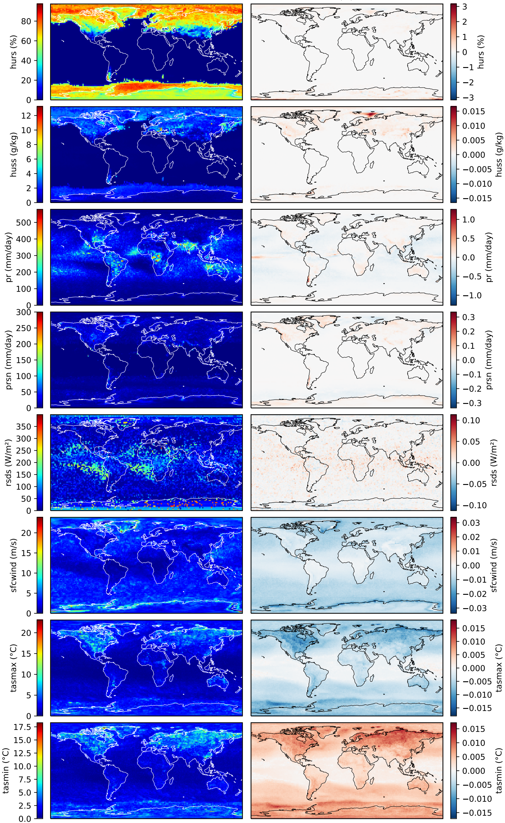
maximum absolute difference over 1850-2014 between data bias-adjusted with v2.4.1 and v2.3(.1) of ISIMIP3BASD
